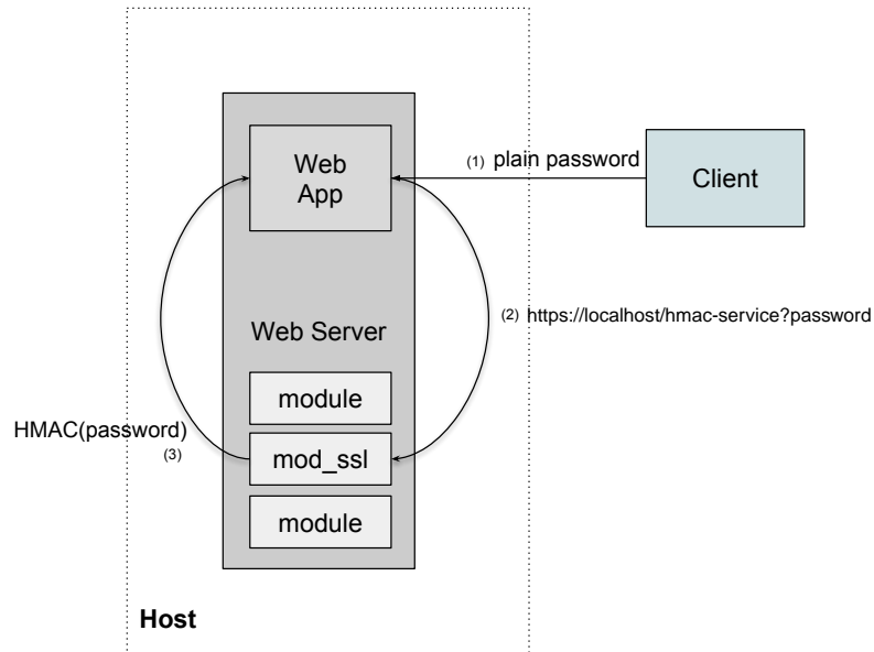
Figure 3.1: Overview of the architecture of modssl-hmac.
