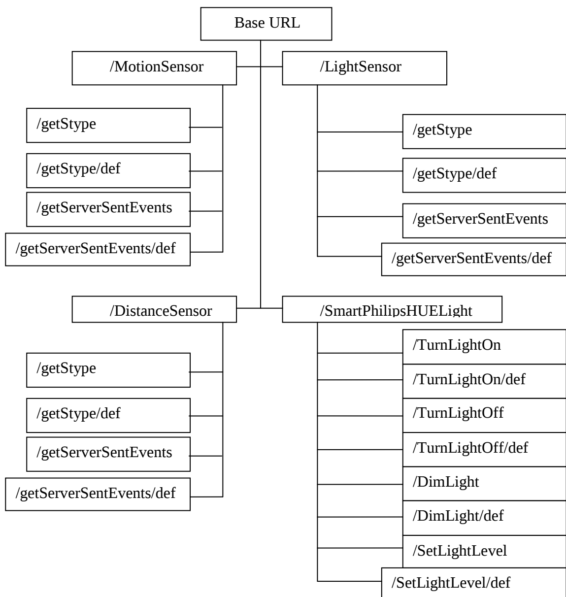
Figure 5.8: List with all available web methods for this demonstration.
