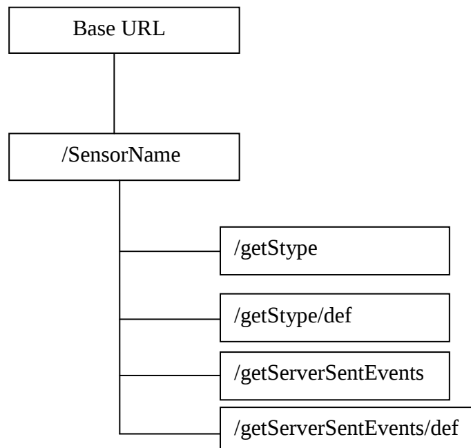
Figure 4.8: Sensor OSGi path general hierarchy.
