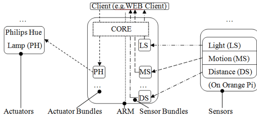
Figure 1.2: General scheme of the system.
