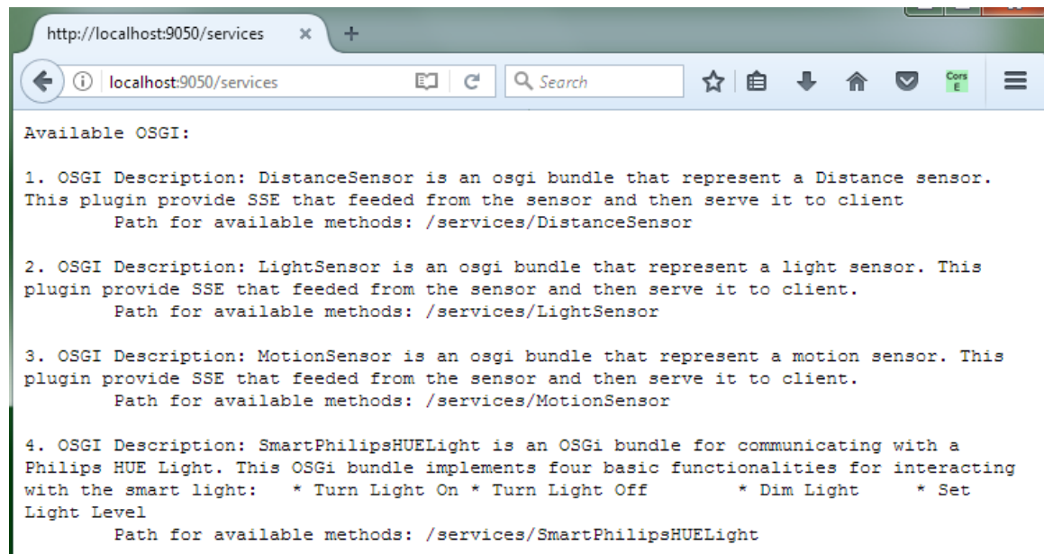
Figure 4.6: List with available OSGi bundles in middleware.
