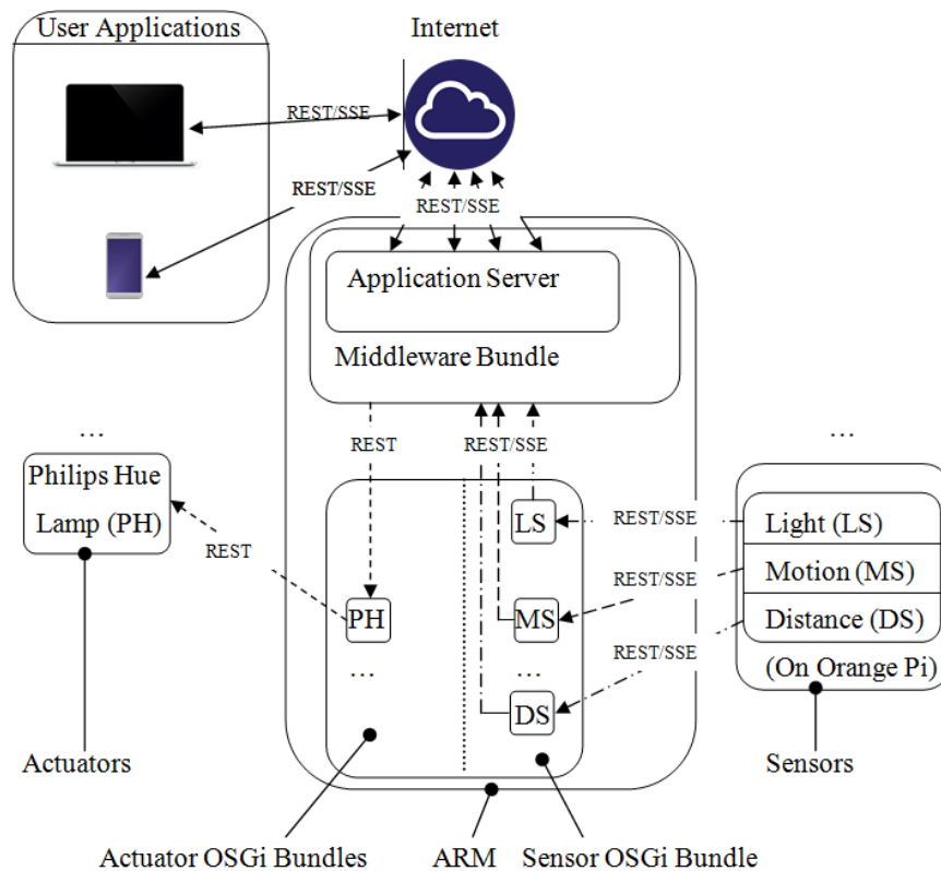
Figure 3.1: General scheme of the system.
