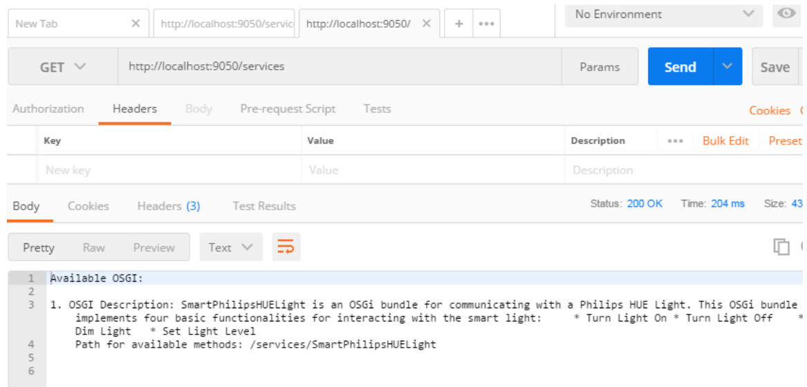
Figure 5.4: Middleware list with available OSGi bundles after Smart Philips Hue Light Installation.
