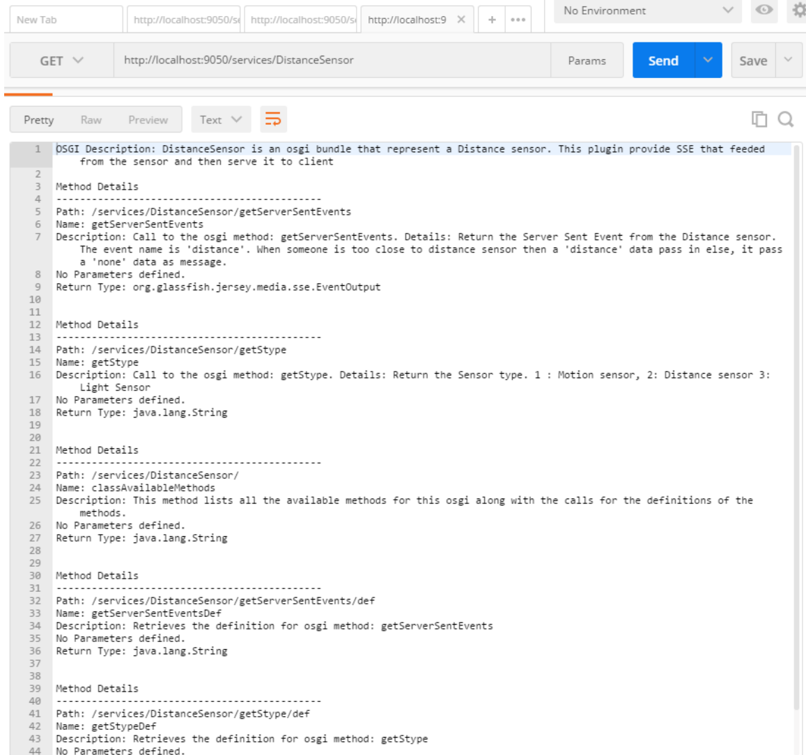
Figure 5.7: Middleware list with available REST & SSE calls for Distance Sensor Bundle.
