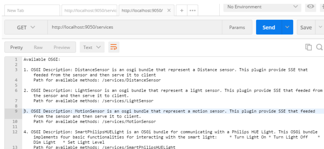
Figure 5.6: Middleware list with available OSGi bundles after Light and Distance Sensor Installation.
