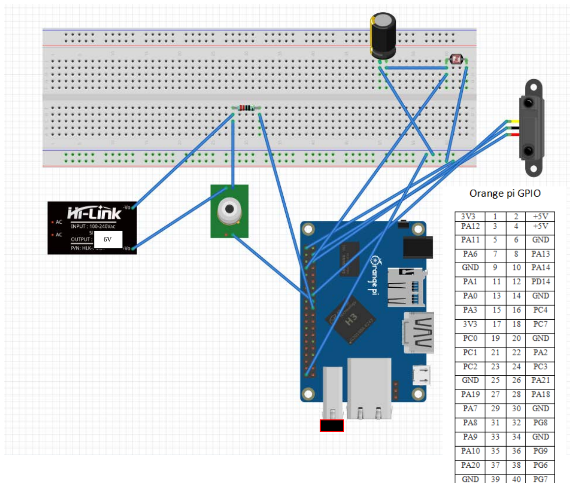
Figure 4.1: Development Board and Sensors hardware connectivity.
