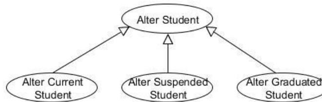
FIGURE 4.2 GENERALIZATION RELATIONSHIPS
