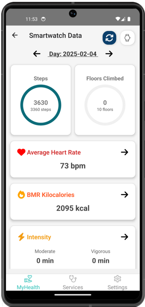
Figure 3.5 Dashboard Screen
