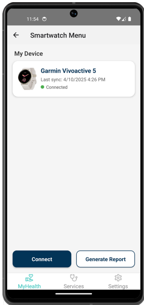
Figure 3.11 Menu Screen
