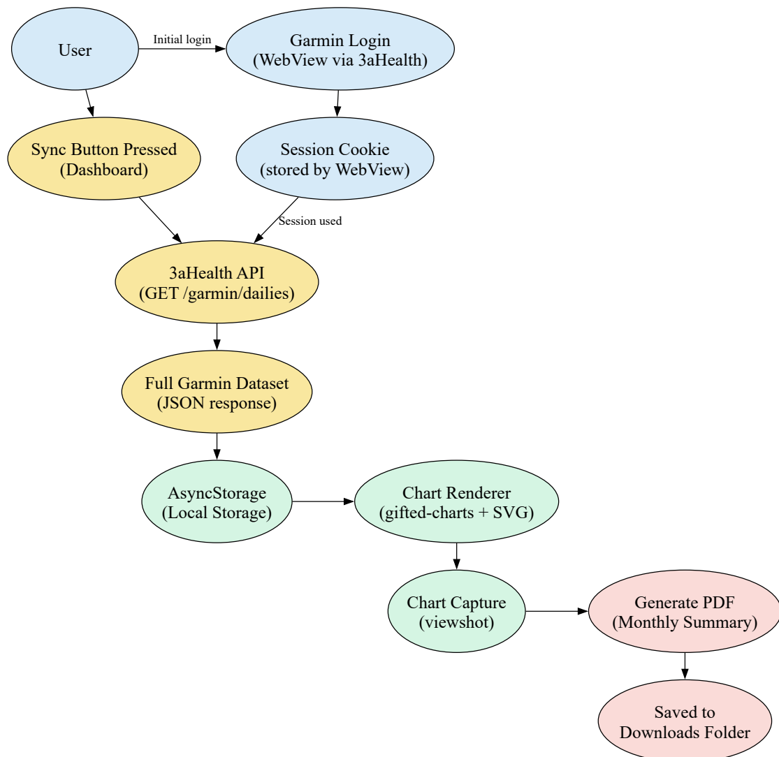
Figure 3.4 Smartwatch Sync and Report Generation Architecture
