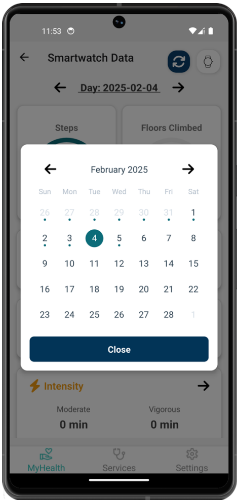
Figure 3.6 Calendar Modal
