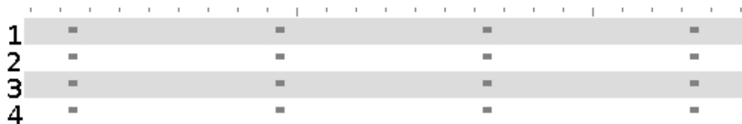
Figure 8: Minimal Schedule
