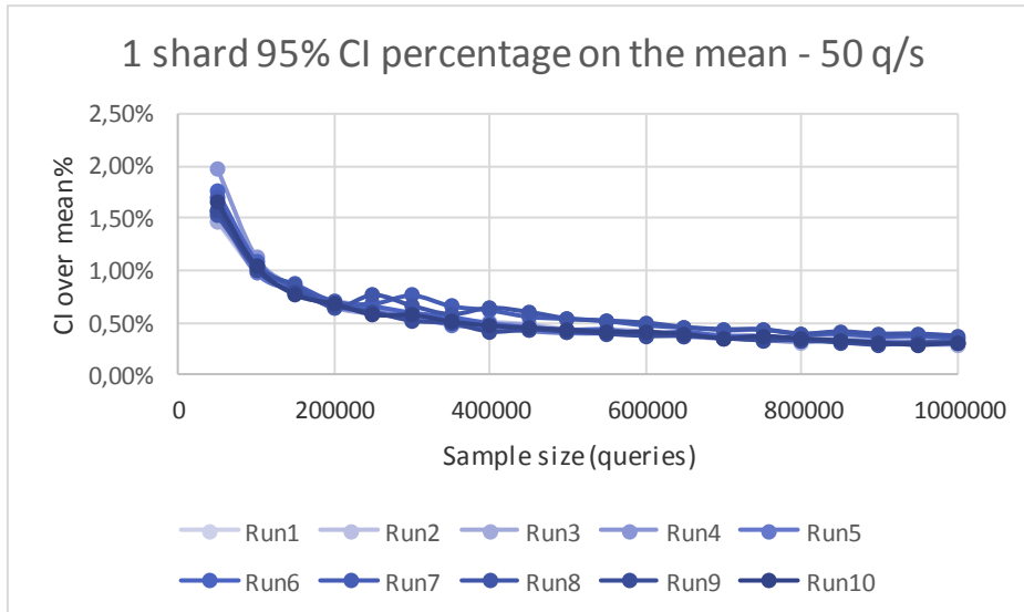
Figure 11. 1 Shard configuration CI over mean at 50 queries per second interarrival rate
