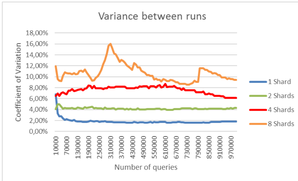
Figure 24. Coefficient of Variation of Tail latency between runs of same shard configuration at 50 queries per second interarrival rate
