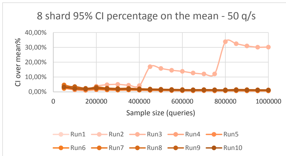
Figure 14. 8 Shard configuration CI over mean at 50 queries per second interarrival rate
