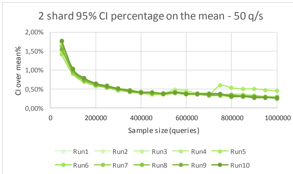
Figure 12. 2 Shard configuration CI over mean at 50 queries per second interarrival rate
