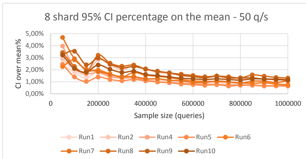
Figure 15. 8 Shard configuration CI over mean at 50 queries per second interarrival rate – no outlier
