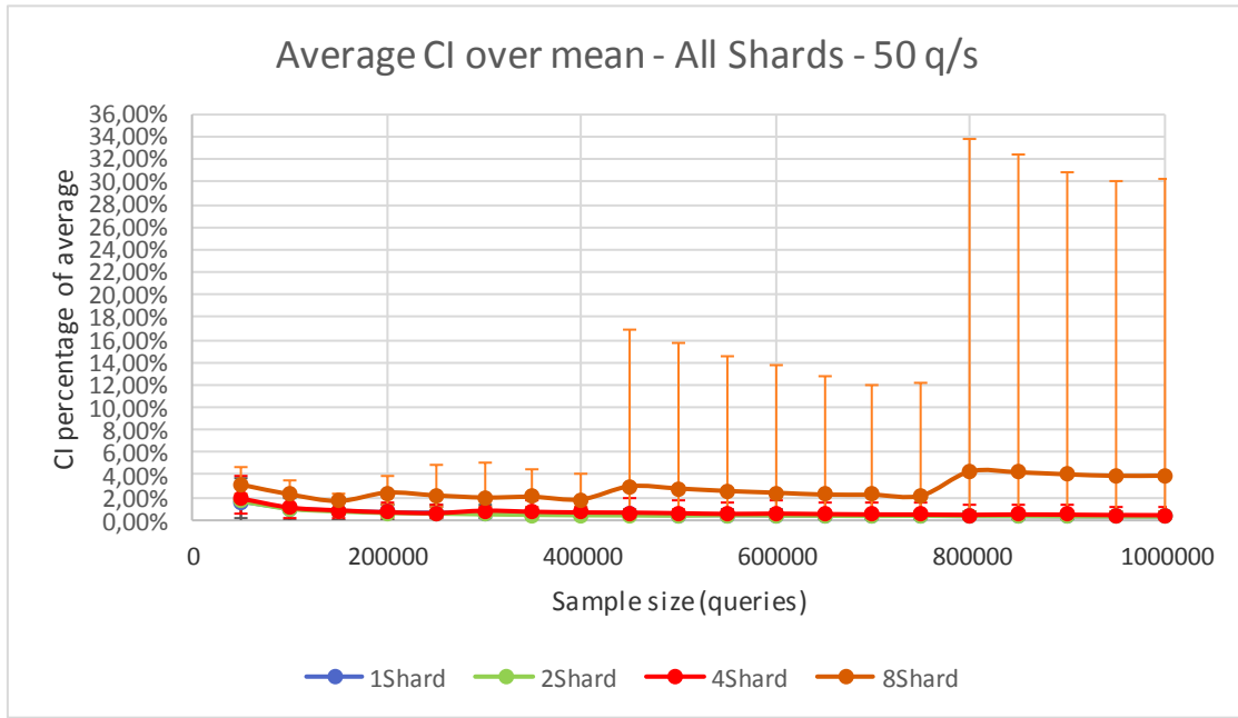
Figure 16. All configurations average CI over mean at 50 queries per second interarrival rate
