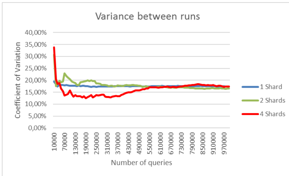
Figure 30. Coefficient of Variation of Tail Latency between runs of same shard configuration at 150 queries per second interarrival rate
