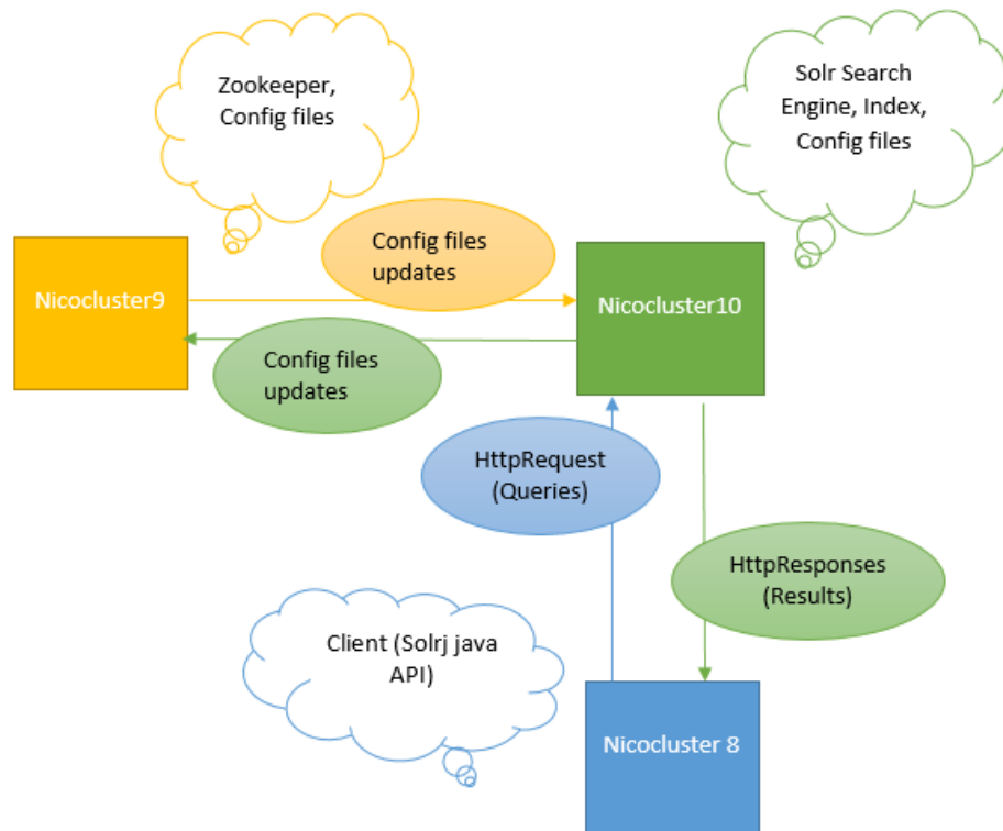
Figure 1. Communication between nodes
