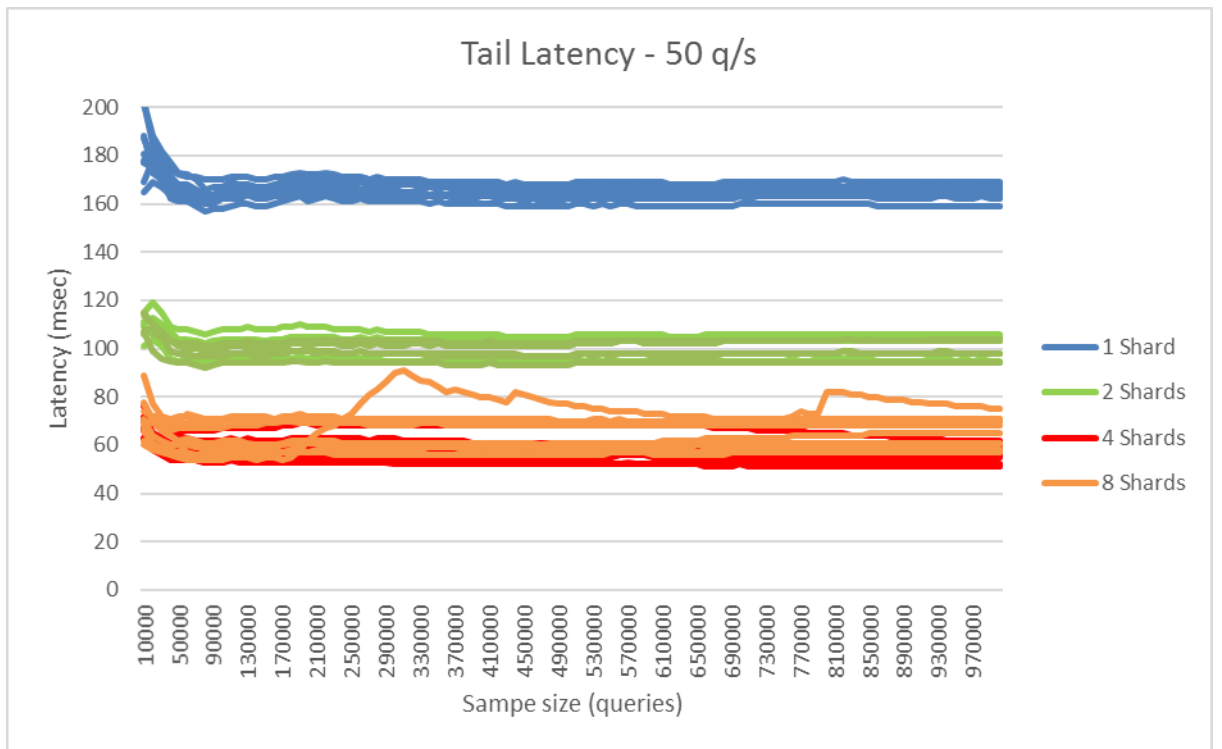
Figure 23. Average Latency at 50 queries per second interarrival rate
