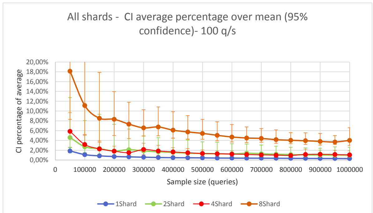
Figure 19. All configurations average CI over mean at 100 queries per second interarrival rate
