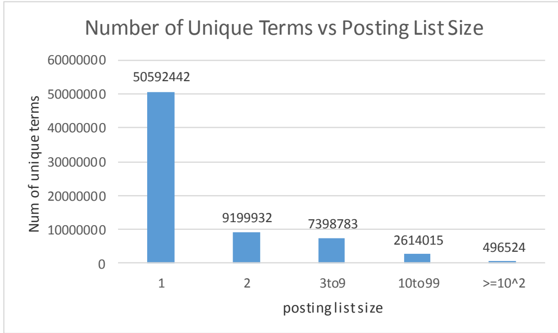
Figure 3. Number of Unique Terms vs Posting List Size
