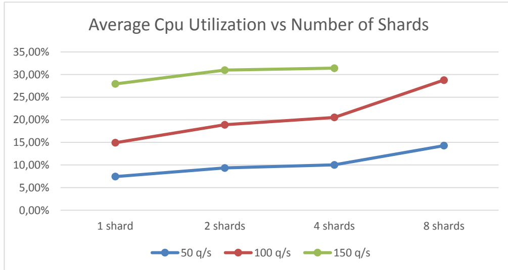
Figure 7. Average CPU Utilization vs Number of Shards for all interarrival rates
