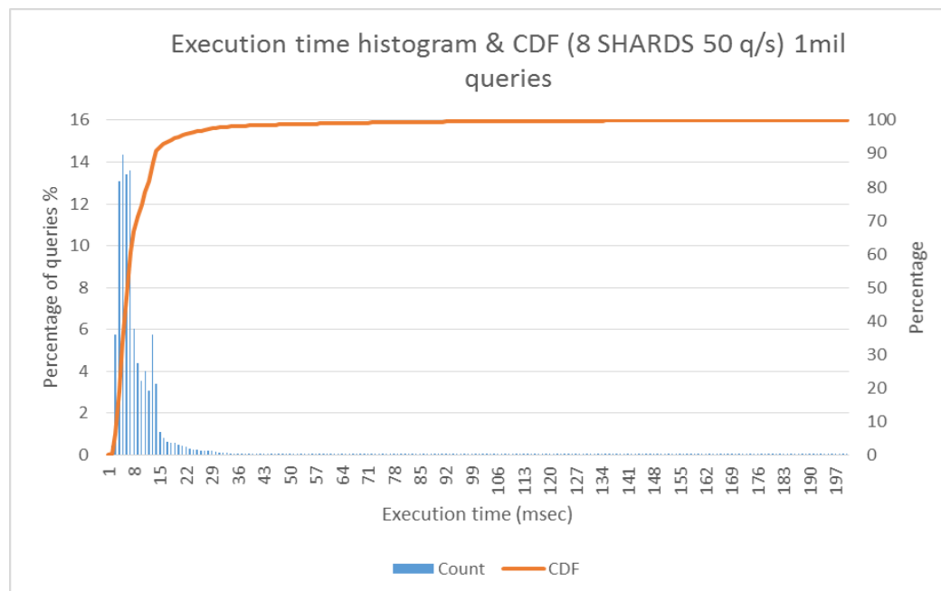
Figure 5. Execution time histogram and CDF of 8 shard configuration at 50 q/s interarrival rate for 1 million queries
