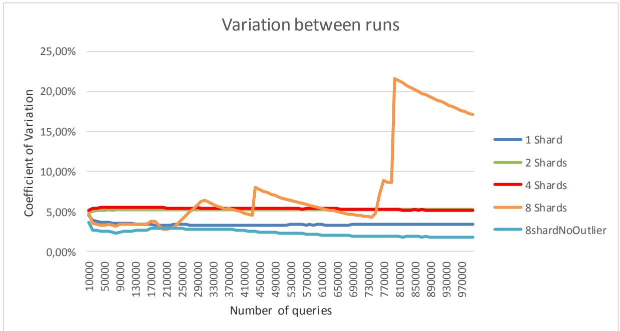
Figure 9. Coefficient of Variation of Average Latency between runs of same shard configuration
