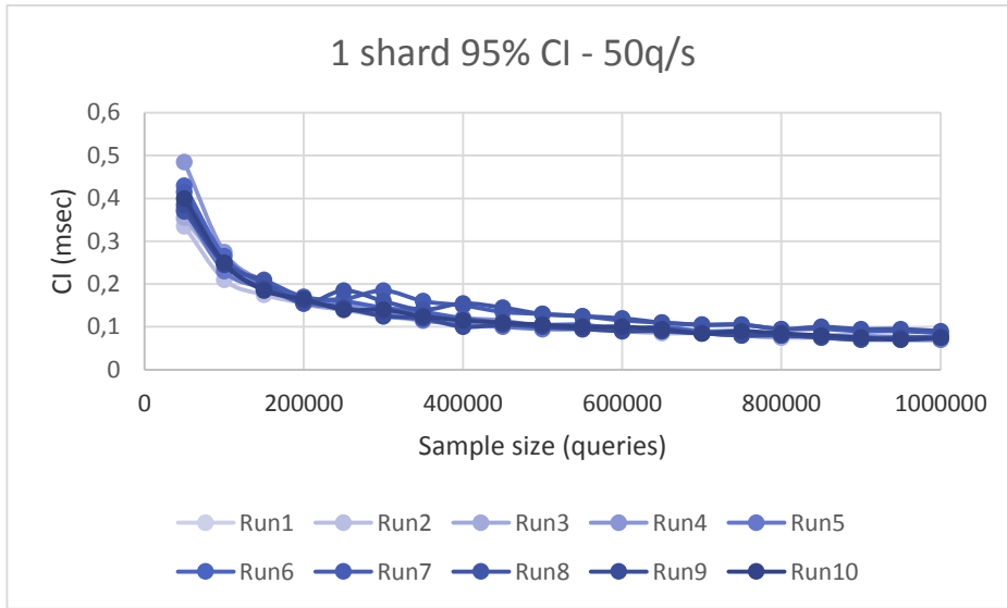
Figure 10. 1 Shard configuration CI at 50 queries per second interarrival rate
