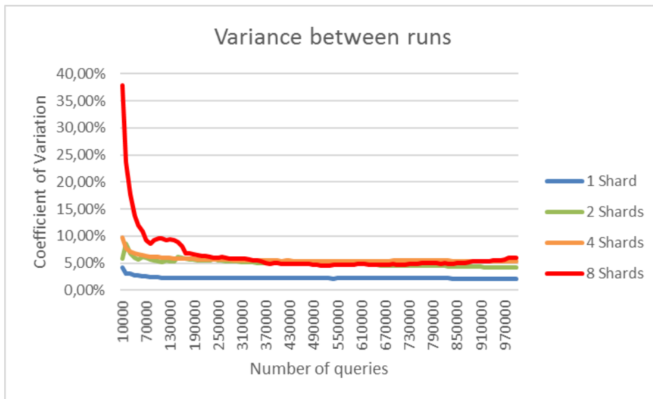
Figure 18. Coefficient of Variation of Average Latency between runs of same shard configuration at 50 queries per second interarrival rate
