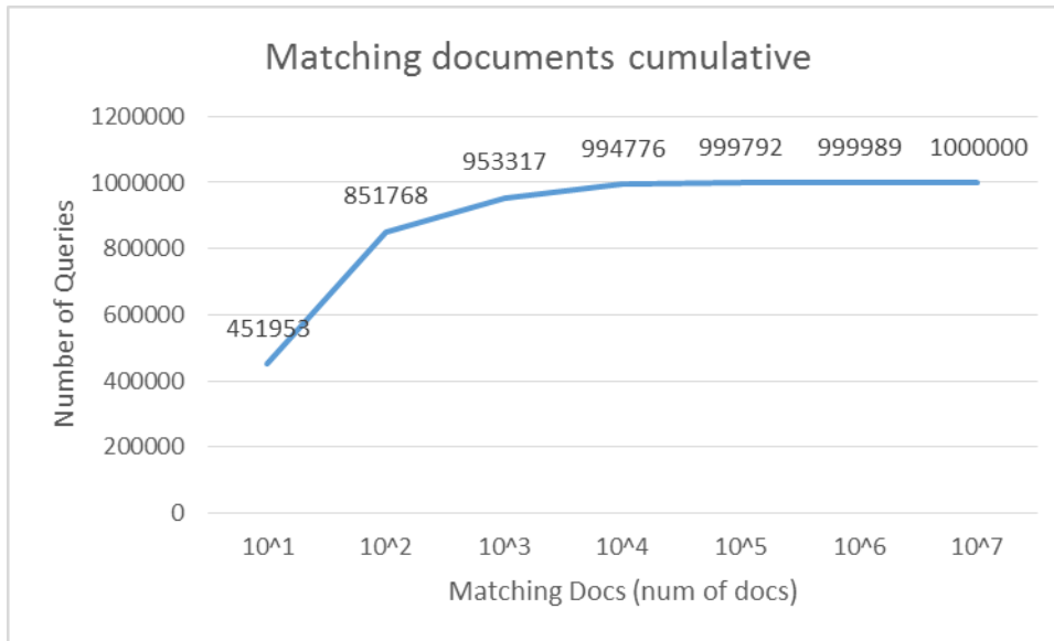
Figure 4. Matching Documents Cumulative
