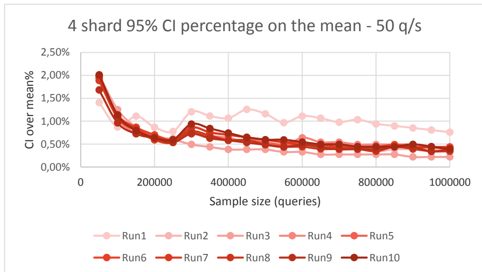
Figure 13. 4 Shard configuration CI over mean at 50 queries per second interarrival rate
