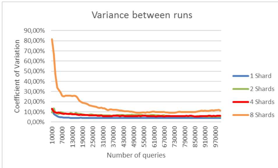
Figure 27. Coefficient of Variation of Tail Latency between runs of same shard configuration at 100 queries per second interarrival rate
