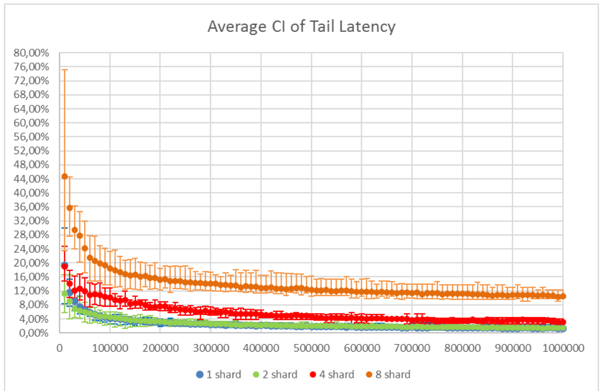
Figure 28. All configurations average CI over Tail at 100 queries per second interarrival rate
