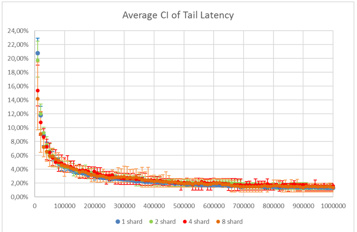
Figure 25. All configurations average CI over Tail at 50 queries per second interarrival rate
