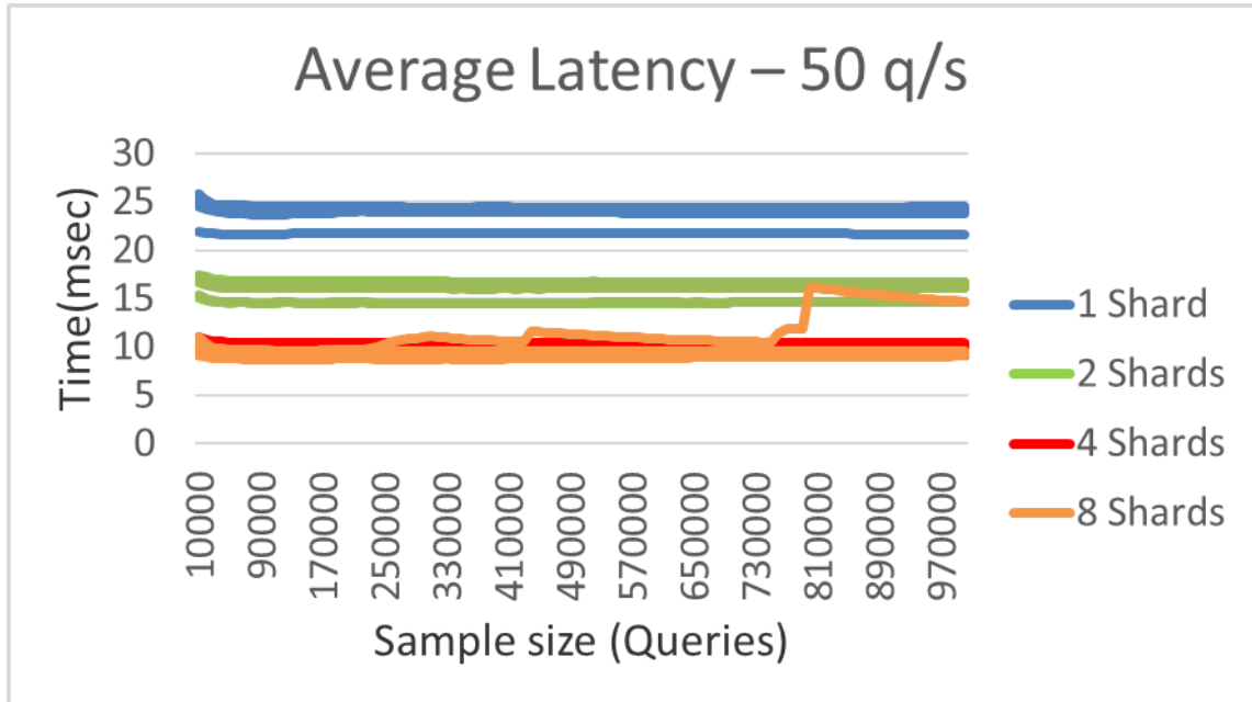
Figure 8. Average Latency at 50 queries per second interarrival rate
