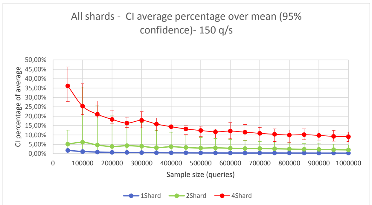
Figure 22. All configurations average CI over mean at 150 queries per second interarrival rate
