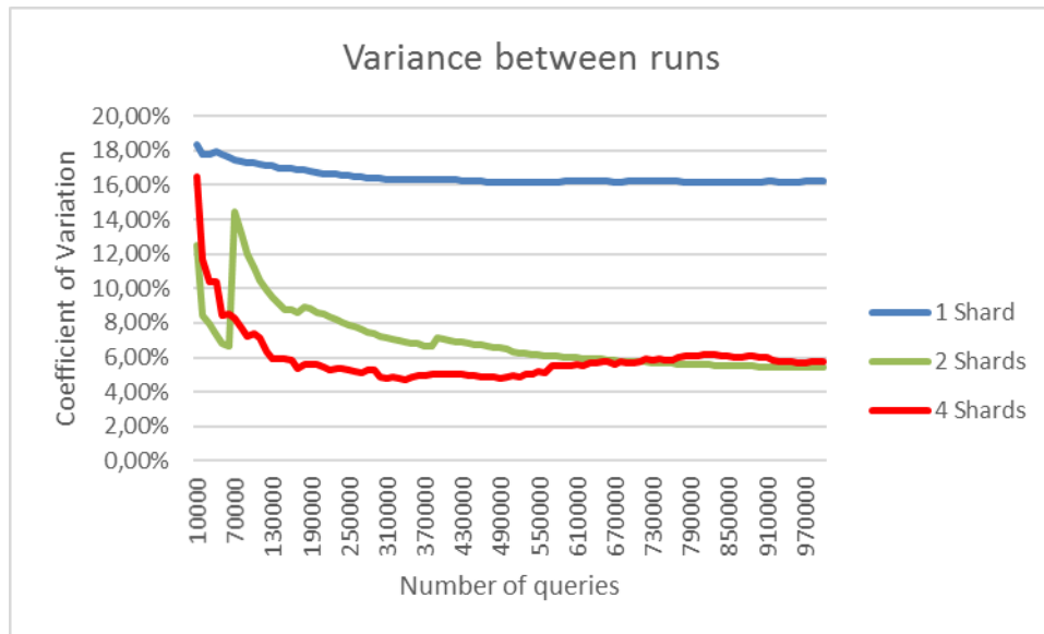
Figure 21. Coefficient of Variation of Average Latency between runs of same shard configuration at 150 queries per second interarrival rate
