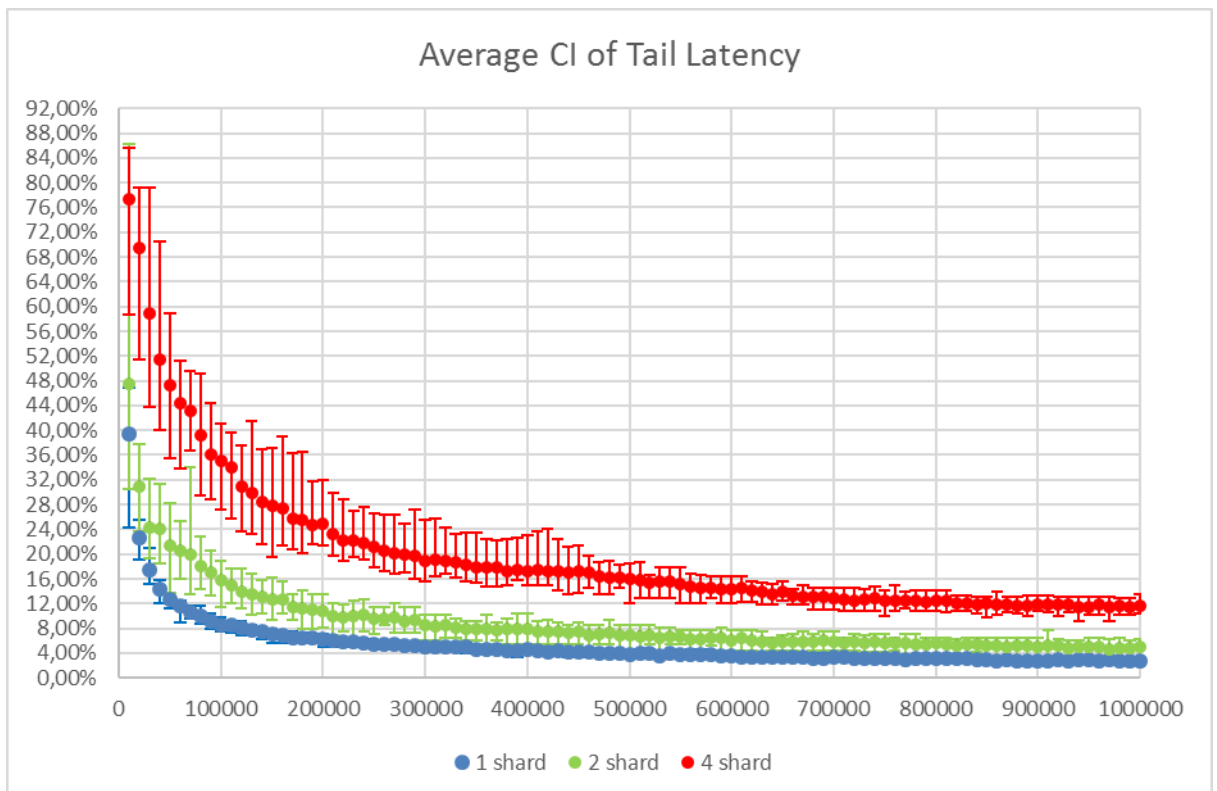
Figure 31. All configurations average CI over Tail at 150 queries per second interarrival rate
